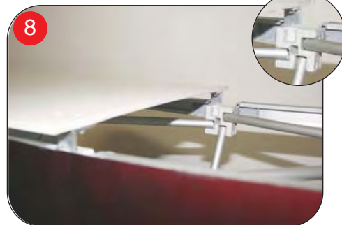
7-8. Install counter tops, inserting hubs securely into routed locations.
